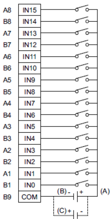
Input Circuit
